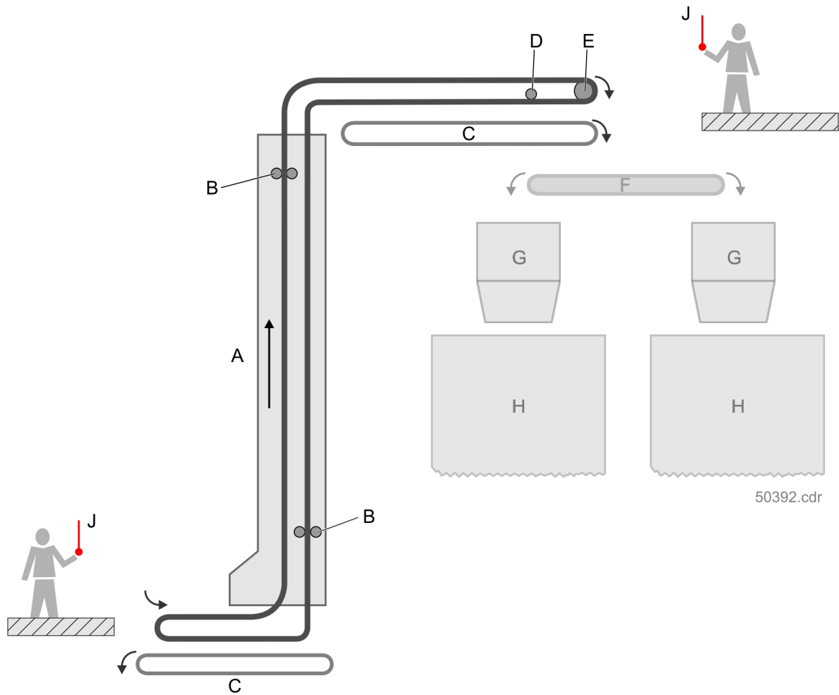
Fig. 16 Corrugated belt conveyor
